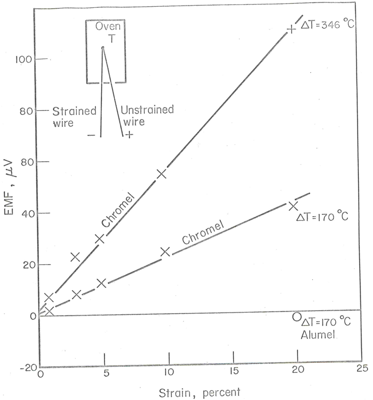
EFFECT OF PERMANANT STRAIN OF THERMOCOUPLE WIRE
